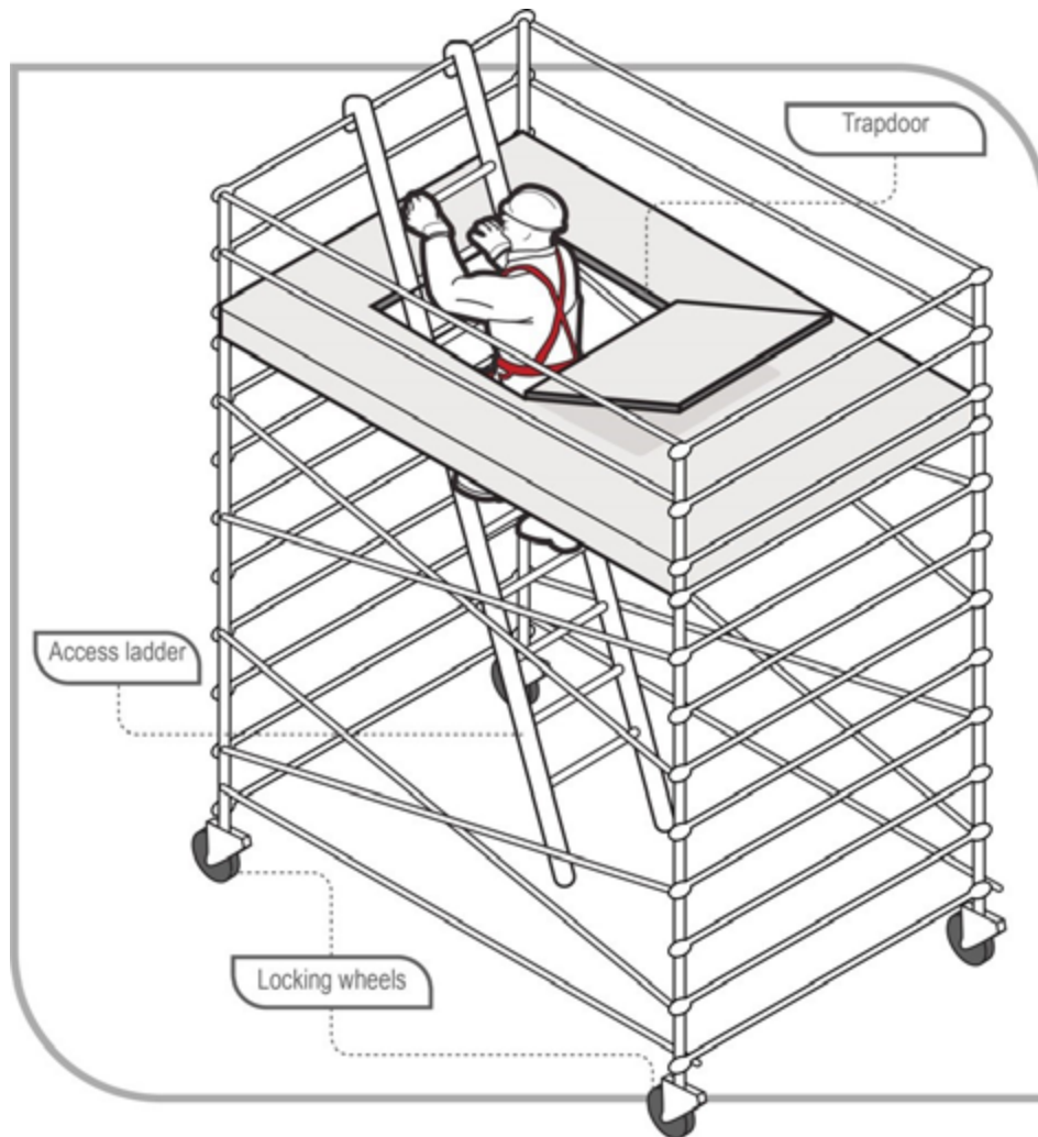
Figure 8 Mobile scaffold with access ladder and trapdoor
