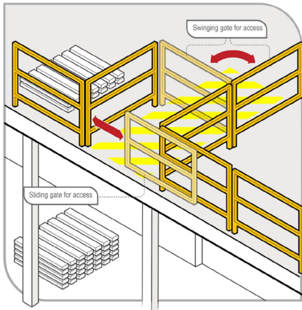
Figure 3 Mezzanine floor barrier
